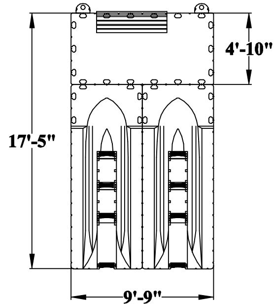
Double EZ Ports with 60"x10' Landing & Bench
